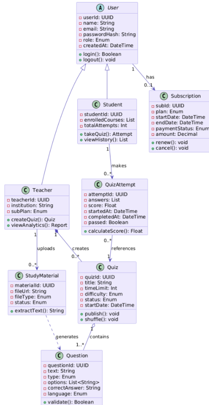
Figure 3: Class Diagram.
